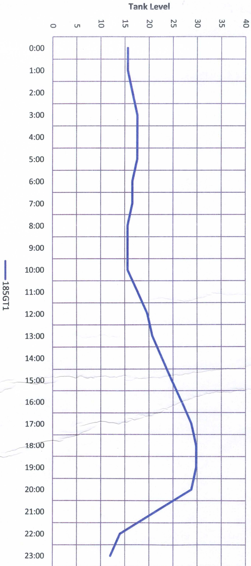
Facility 185 Tank Level August 19, 2009
