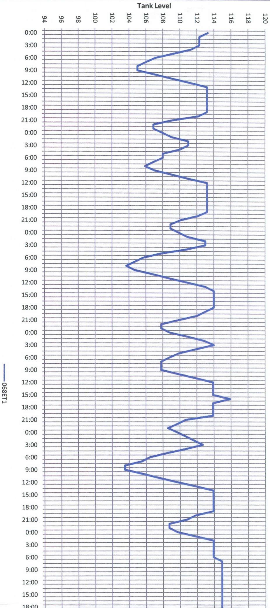
Facility 068 Tank Level August 17, 2009 to August 23, 2009
