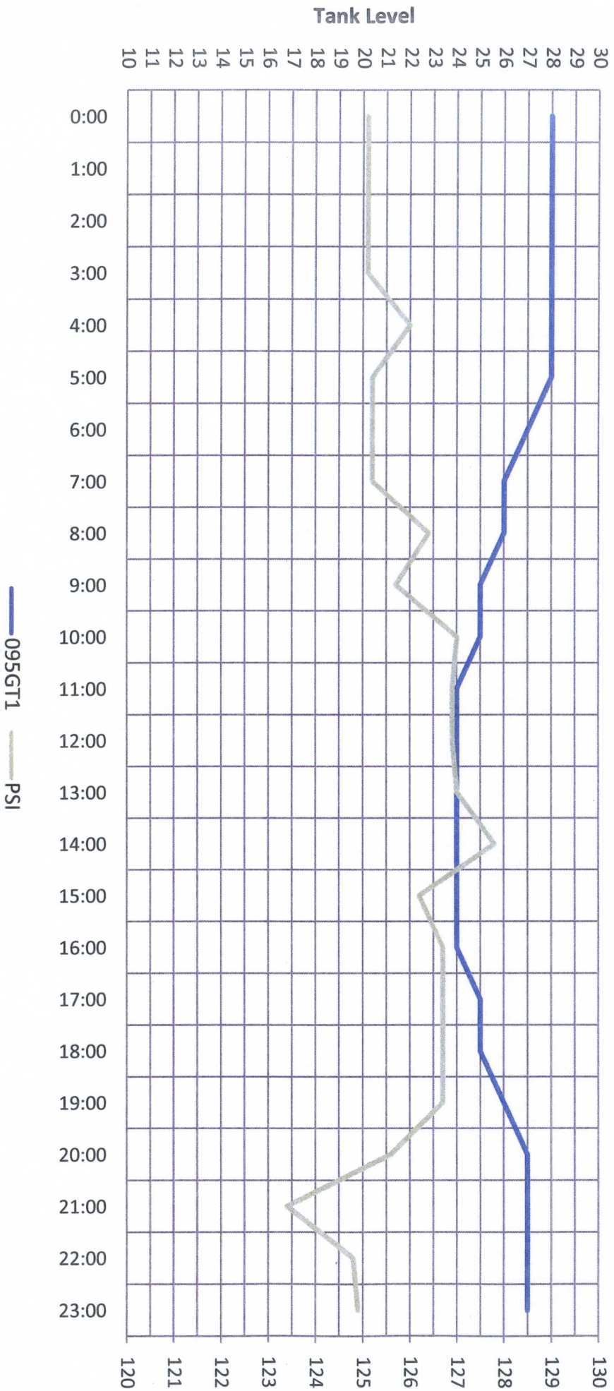
Facility 095 Tank Levels August 17, 2009
