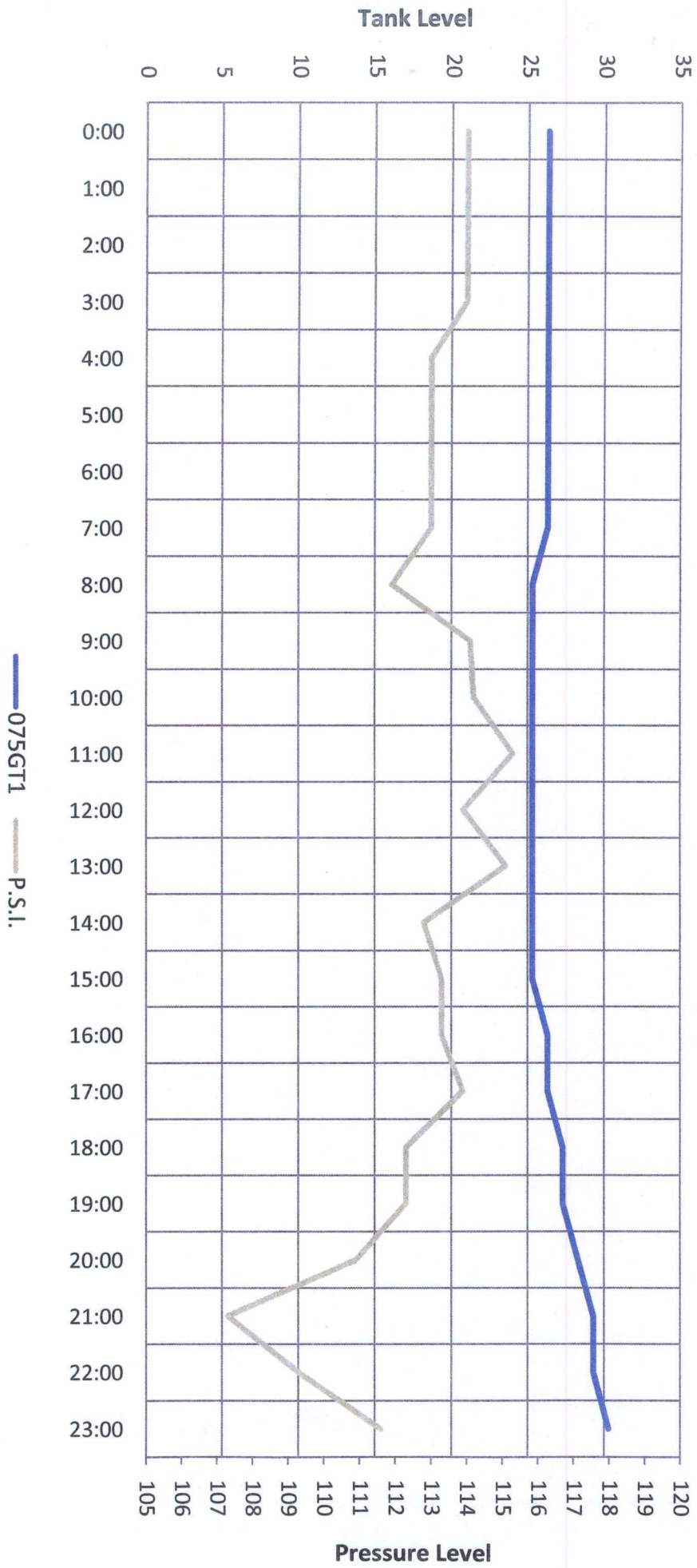
Facility 075 Tank & Pressure Levels August 21, 2009
