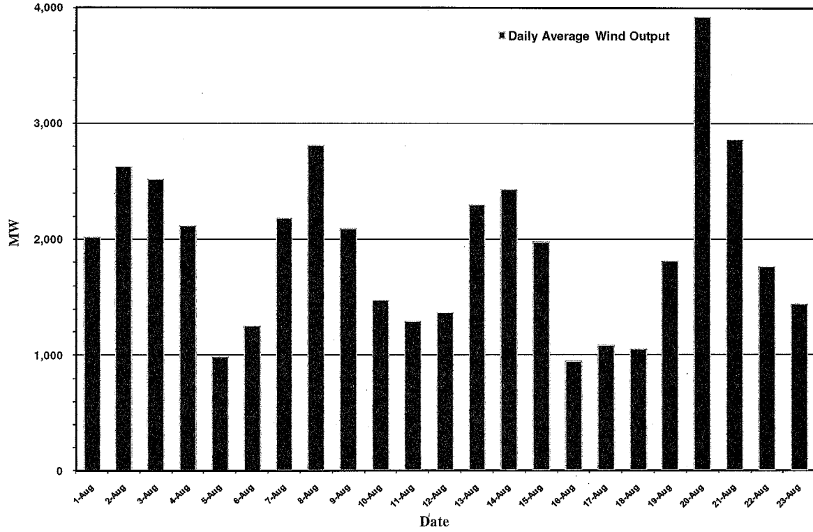
August 2010 Daily Average Wind Output
